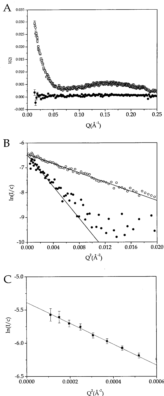
FIGURE 3 ( A ) Scattering profile of (●) 33.3 mM DDMAB in 200 mM NaCl, 50 mM \text{Na}_2\text{HPO}_4/\text{NaH}_2\text{PO}_4 , pH = 7.9 solution after a buffer subtraction; (○) 8.77 mg/mL SN/GpA99 in 33.3 mM DDMAB after subtraction of detergent solution as background; (□) 8.77 mg/mL SN/GpA99 in 33.3 mM DDMAB after subtraction of buffer as background. ( B ) Guinier plot of (○) 5.4 mg/mL SN in buffer solution; (●) 4.7 mg/mL SN in 33.3 mM DDMAB solution. ( C ) Guinier plot of 8.77 mg/mL SN/GpA99 in 33.3 mM DDMAB, 200 mM NaCl, 50 mM \text{Na}_2\text{HPO}_4/\text{NaH}_2\text{PO}_4 , pH = 7.9 solution. R_g = 65 \pm 4 \text{ \AA} .
